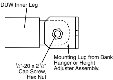
1400 Leg-to-Bank Assembly attachment.
