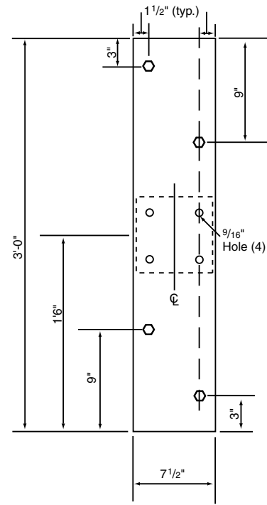
3' Wood Wall Pad
