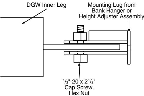
1500 Leg-to-Bank Assembly attachment.
