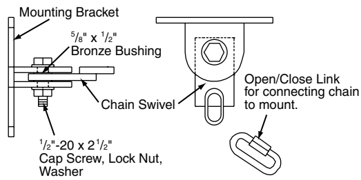
Wall Mount for 1500 chain supports.
