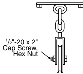
Cable Sheave for 1400.
