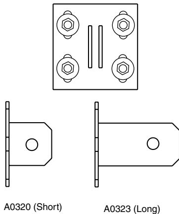
Mounts for 1400.
