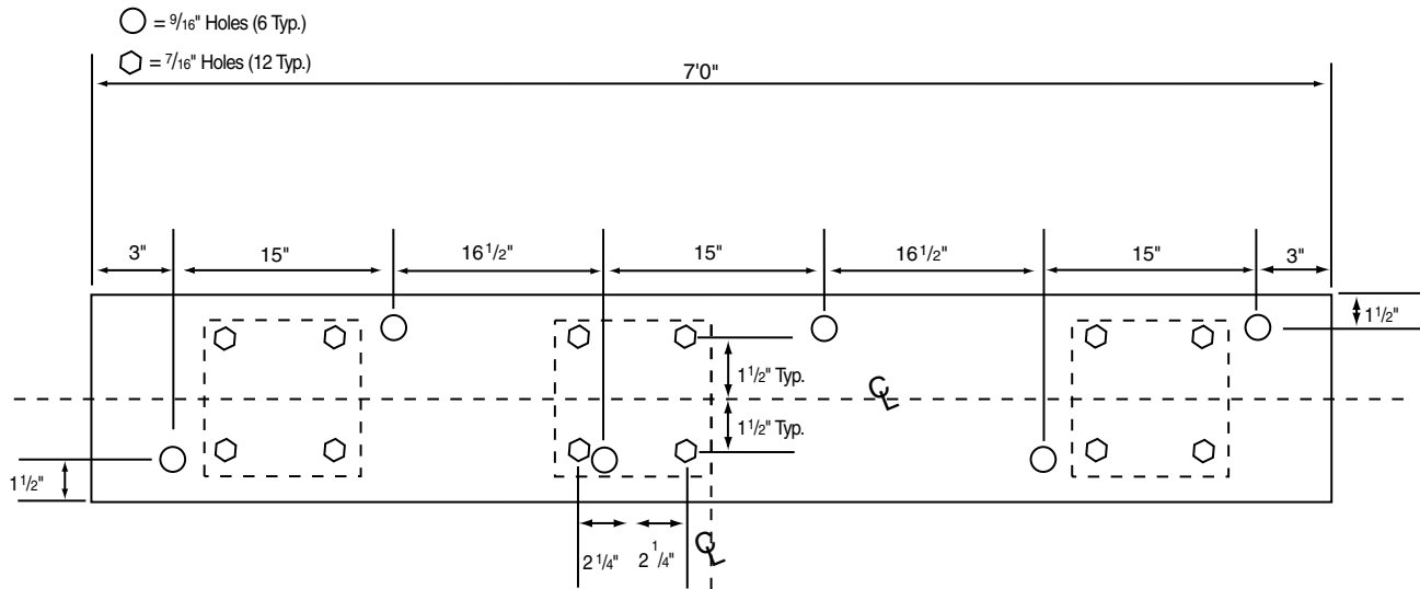
7' Wall Pad (for use with 1400)
