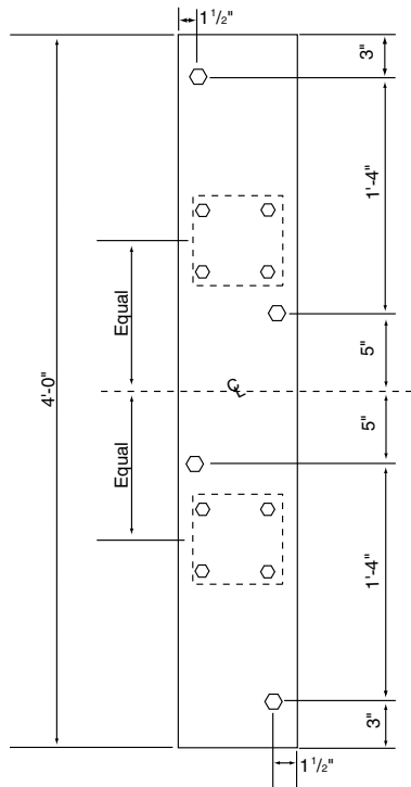
4' Wall Pad
