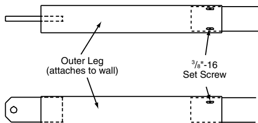
Leg for 1400 and 1500.
