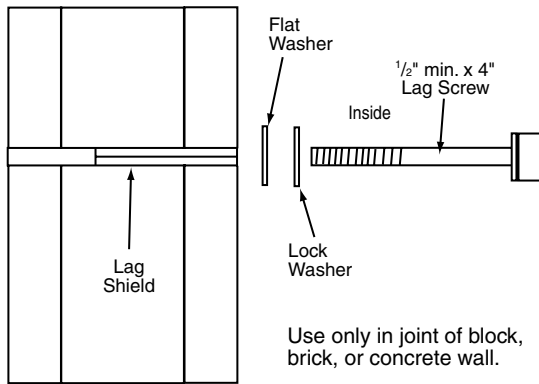
Lag Screw with Lag Shield
