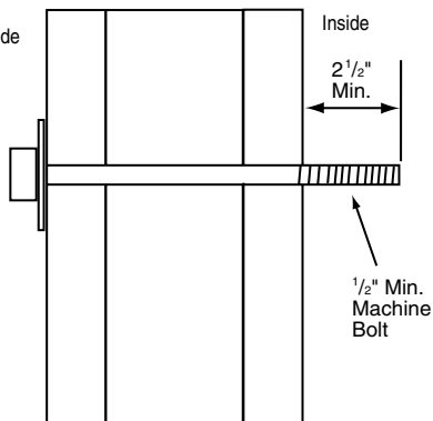
Through Bolt
