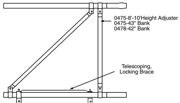
Example of vertical braces on Wall-Mount Frames (side view), including 1500 telescoping, locking brace.
