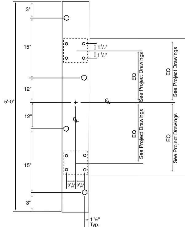
5' Wall Pad
