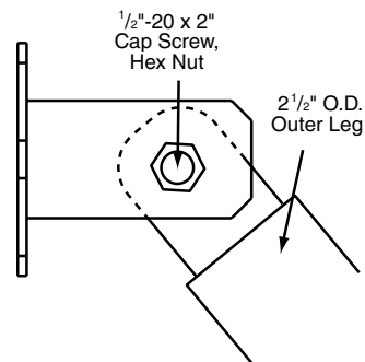
(For attachment of horizontal Braces, including movable, locking Kick Brace on 1500).
