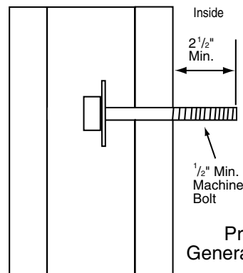
Set-in Bolt
