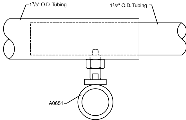
(For attachment of horizontal Braces, including movable, locking Kick Brace on 1500).
